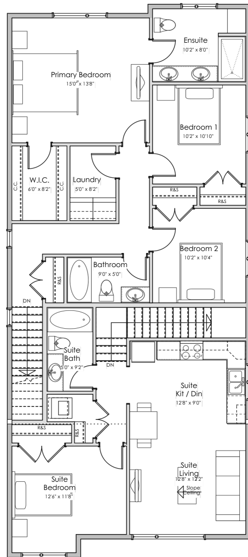
UPPER FLOOR: 1551 sq.ft.
