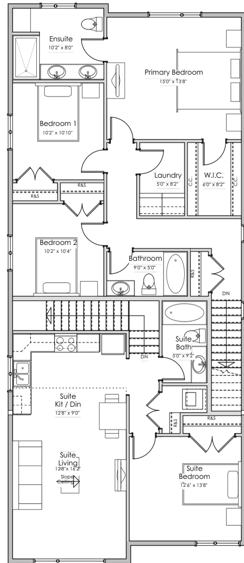
UPPER FLOOR: 1615 sq.ft.
