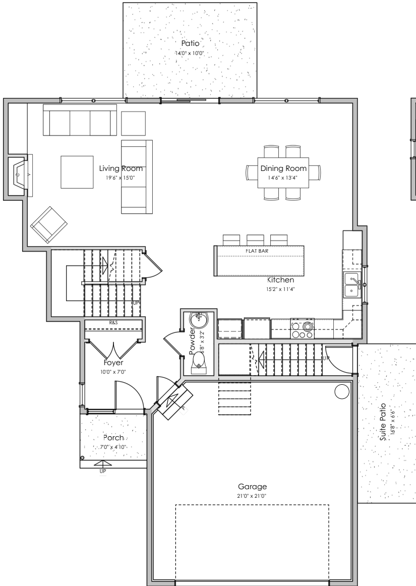
MAIN FLOOR: 1032 sq.ft.
