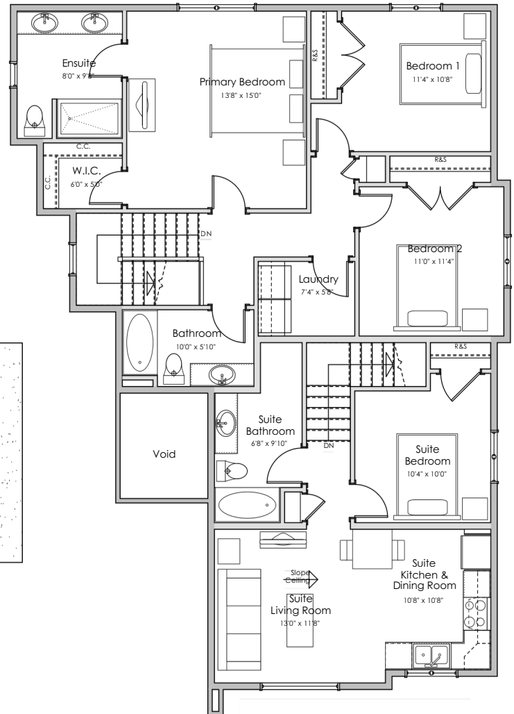
UPPER FLOOR: 1427 sq.ft.
